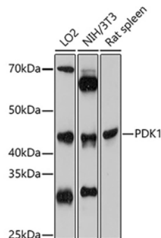
Fig. 1. Western blot analysis of extracts of various cell lines, using PDK1 antibody at 1:3000 dilution. Secondary antibody: HRP-labeled Goat Anti-Rabbit IgG(H+L) (A0208) at 1:1000 dilution. Lysates/proteins: 25µg per lane. Blocking buffer: QuickBlock™ Blocking Buffer (P0231). Detection: BeyoECL Star (P0018A). Exposure time:1s.
